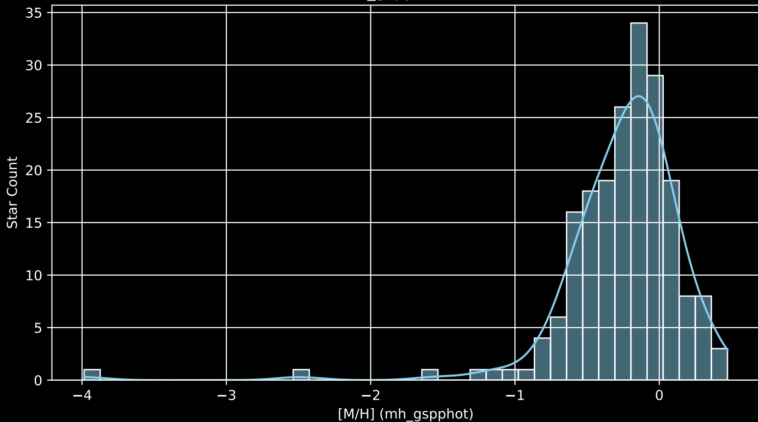
APOGEE DR17 Field: [133-63_MGA [M/H] (mh_gspphot) (n= 197)
