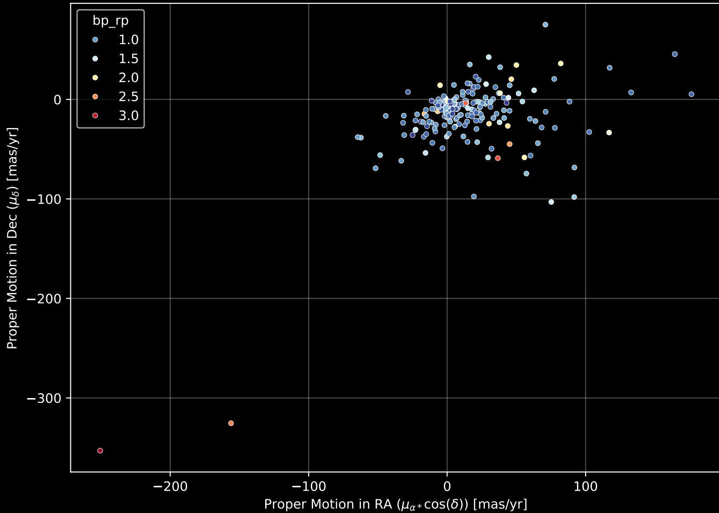
APOGEE DR17 Field: [133-63_MGA] Proper Motion Diagram (n= 198)
