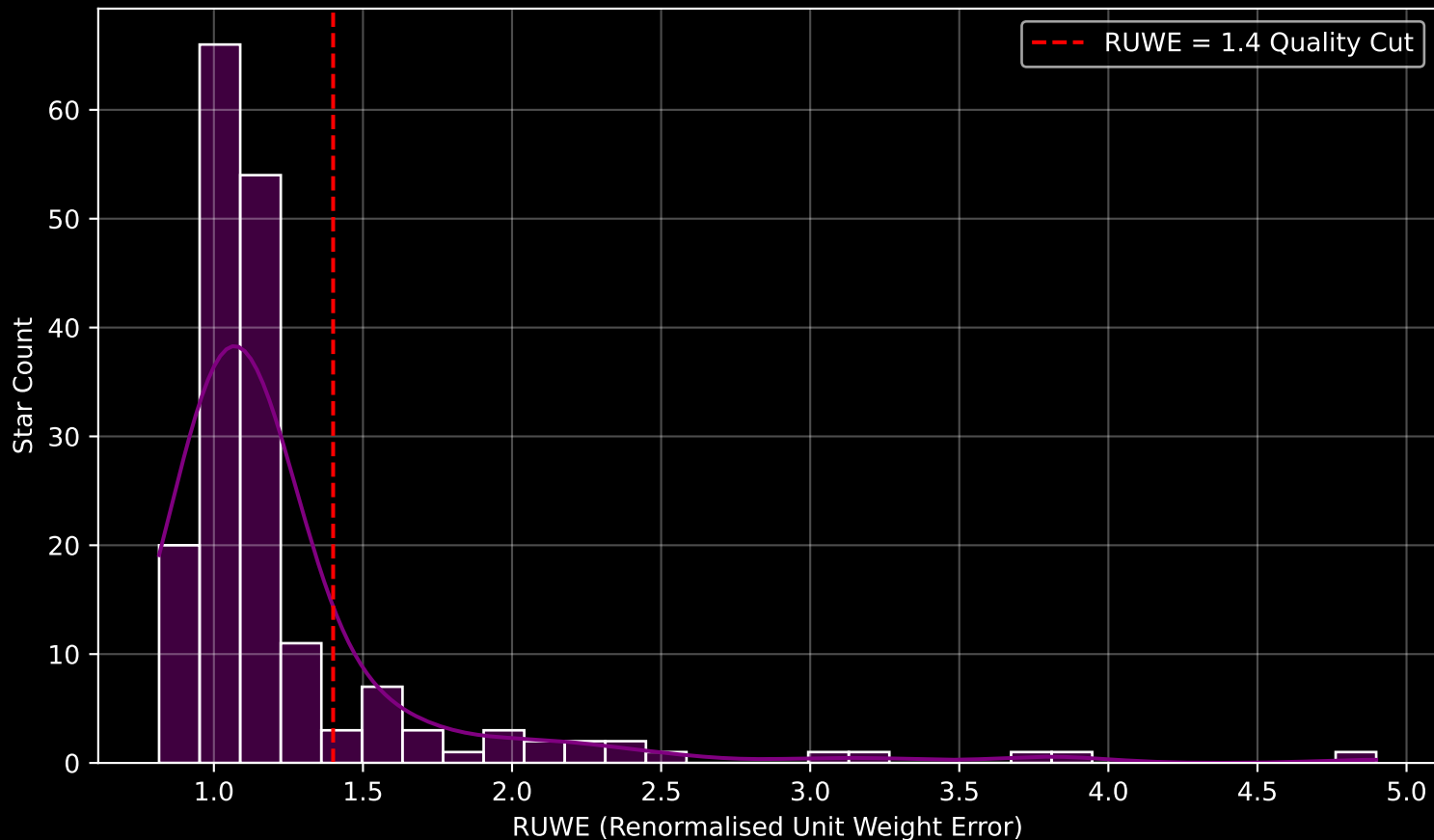
GAPOGEE DR17 Field [133-63_MGA] RUWE Distribution (n= 180)
