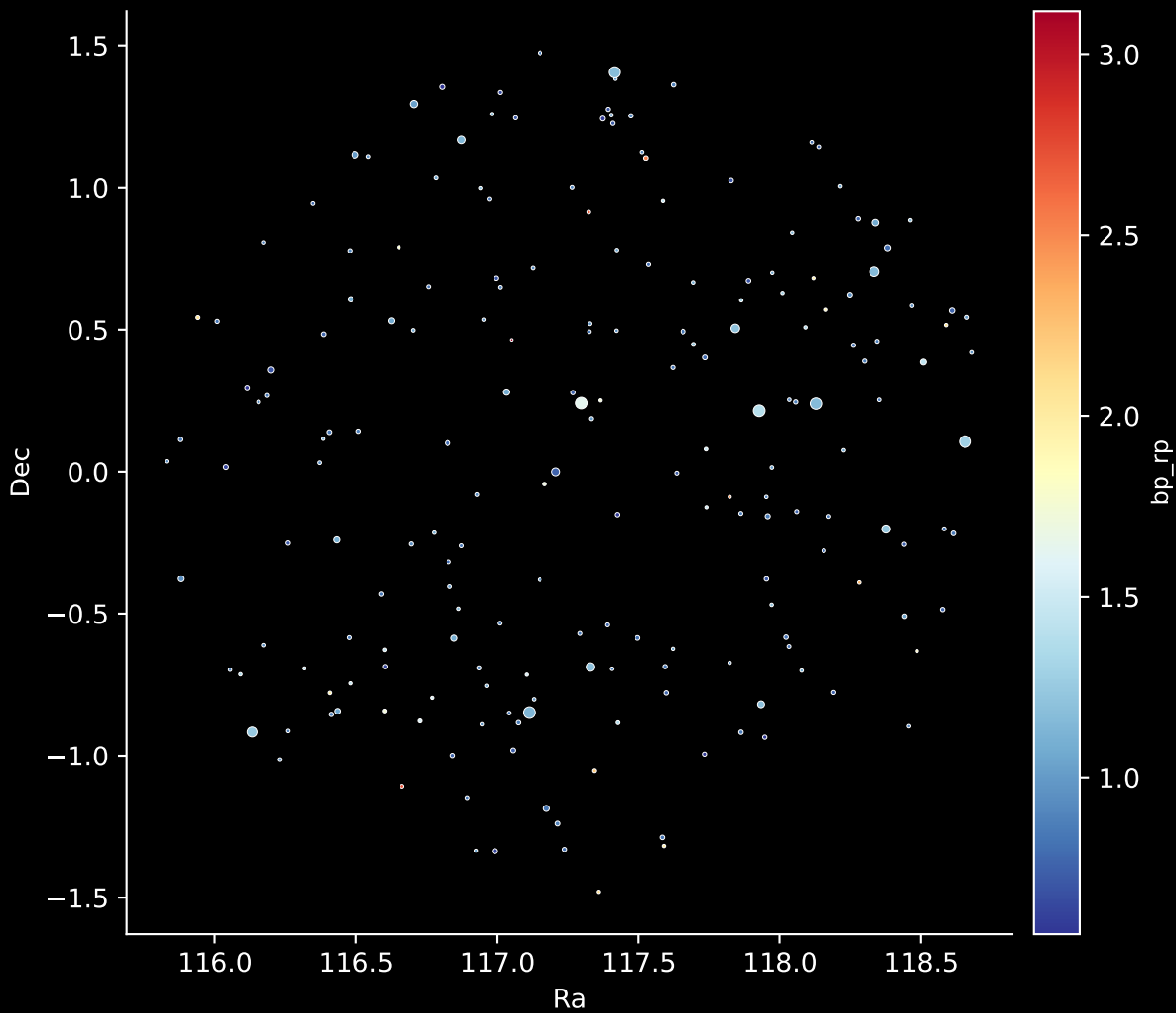
APOGEE DR17 Field: [133-63_MGA] Stars: 198
