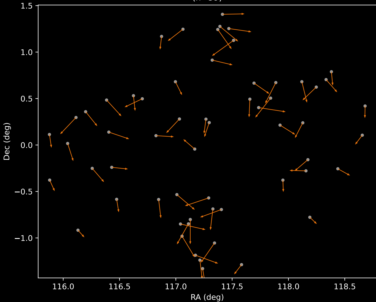
APOGEE DR17 Cluster 2 Proper Motion Vectors (n=59)
