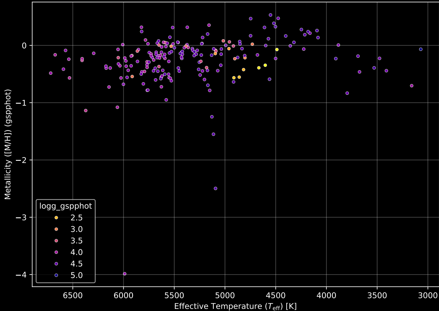
APOGEE DR17 Field: [133-63_MGA] Stellar Population Parameters (n= 198)
