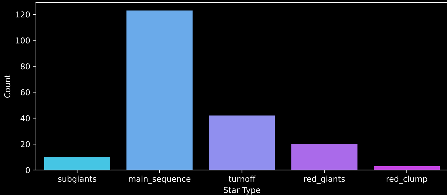
APOGEE DR17 Field: [133-63_MGA] Count plot of Star Type
