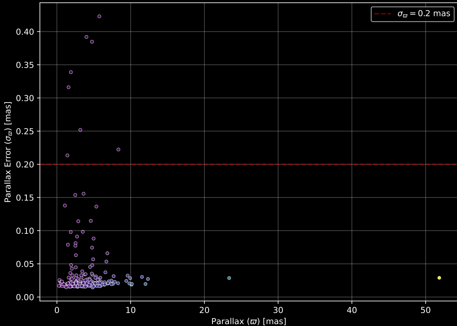
APOGEE DR17 Field: [133-63_MGA] Parallax Quality (n= 198)
